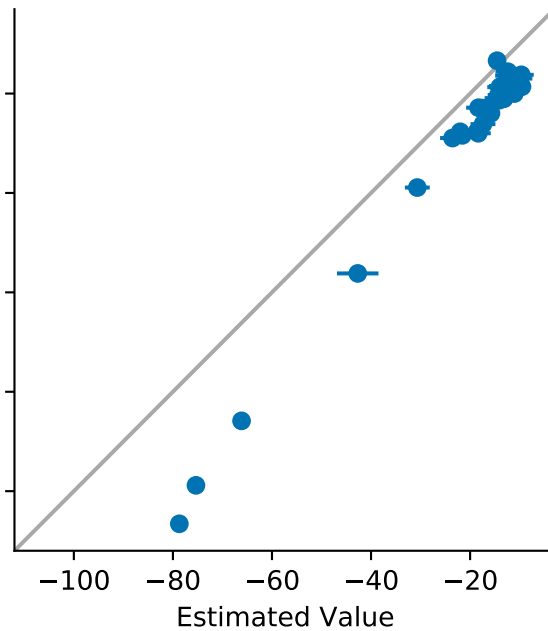
FreeSolv ROH OpenFF 1.2.0
