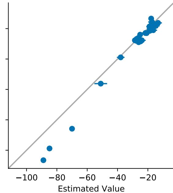
FreeSolv ROH after perturb_32 BCC Fit
