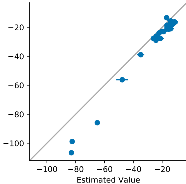
FreeSolv ROH after BCC Fit
