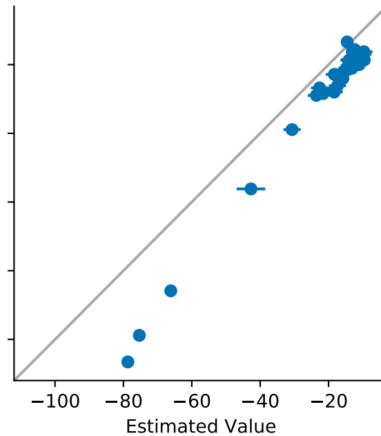
FreeSolv ROH after perturb_5 BCC Fit
