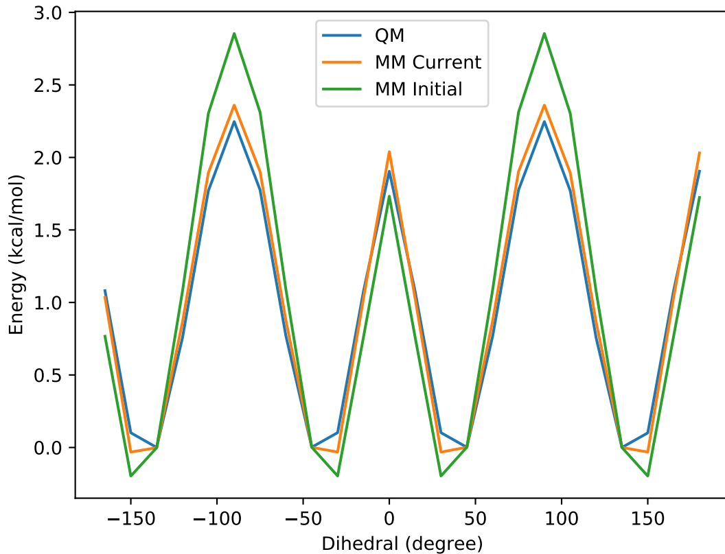
Torsion profile: iteration 3 System: c1ccc(cc1)c2cccc(c2)Cl-torsiondrive1d-0
